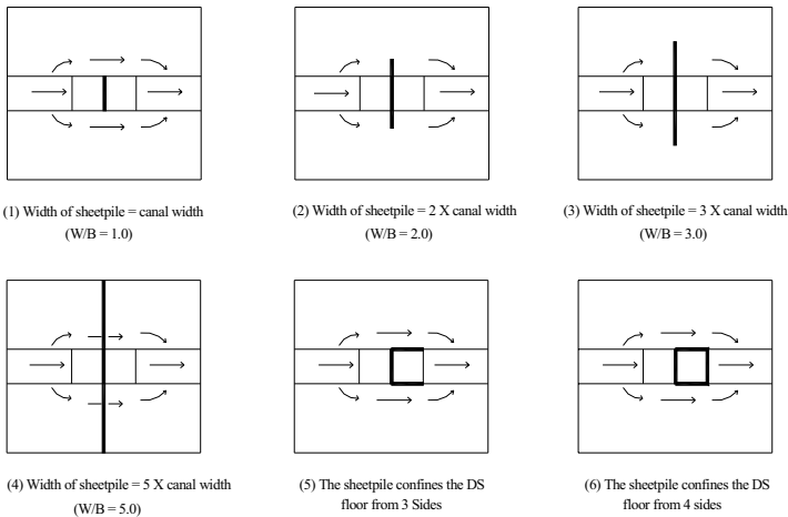
Figure 2. Different arrangements for sheetpile driven under the structure.
