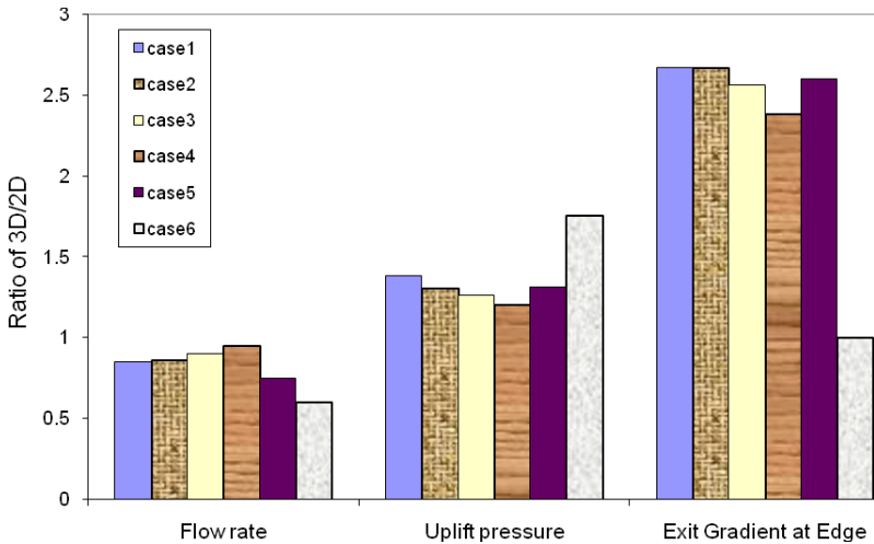
Figure 4. Change of flow rate, uplift pressure, and exit gradient with sheetpile configurations.
